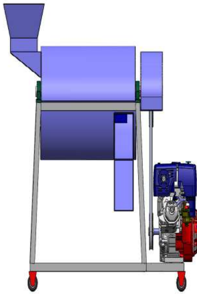
Tampak Samping
