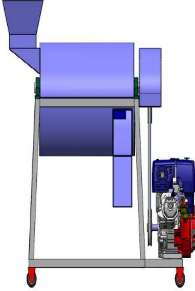
Tampak Samping
