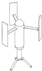
Gambar 1. Tampak Perspektif Turbin full
