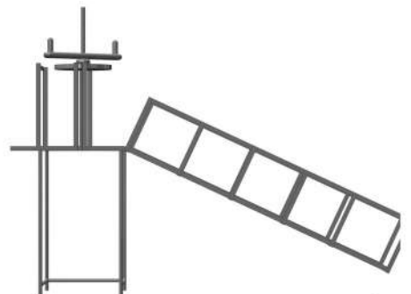
Tampak Samping
