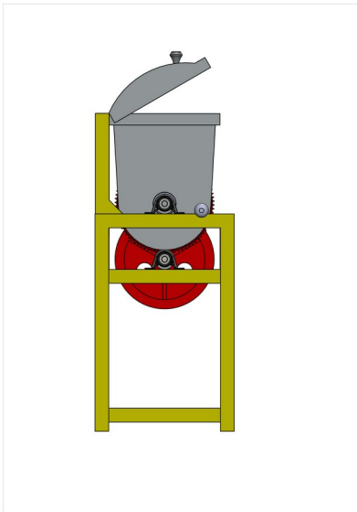
Tampak Samping
