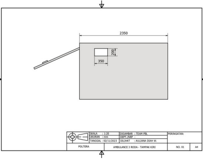
Tampak Samping
