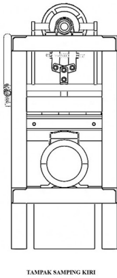
TAMPAK SAMPIING KIRI
