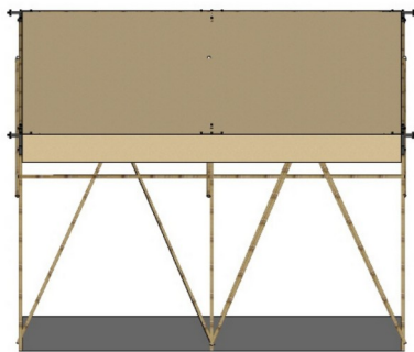
Tampak Samping Kiri
