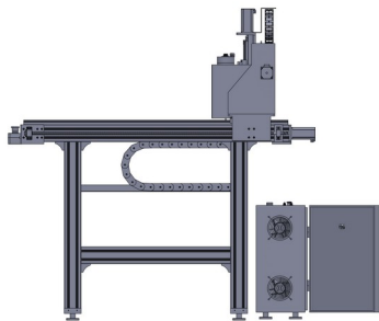
Tampak Samping
