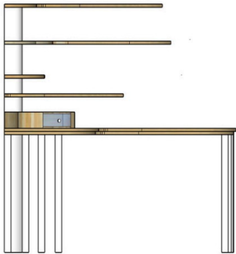
Tampak Samping
