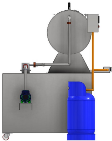
Tampak Samping
