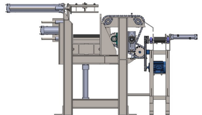
Tampak Samping
