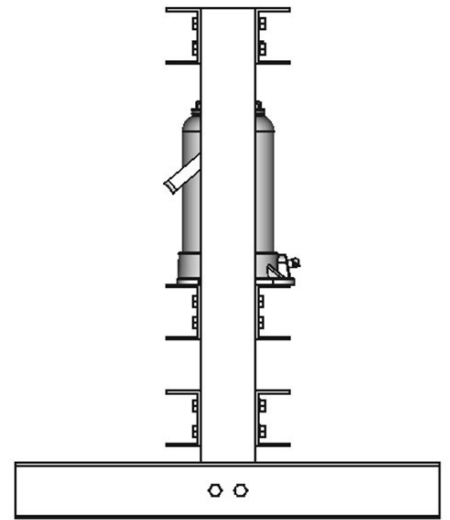
Tampak Samping
