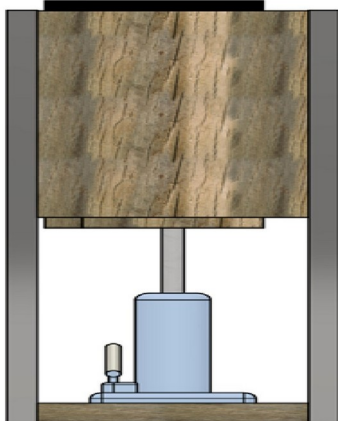
Tampak Samping
