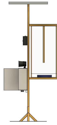
Tampak Samping
