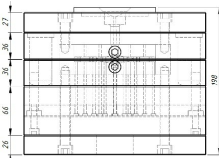
Tampak Samping
