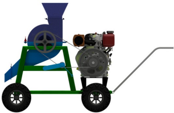
Tampak Samping
