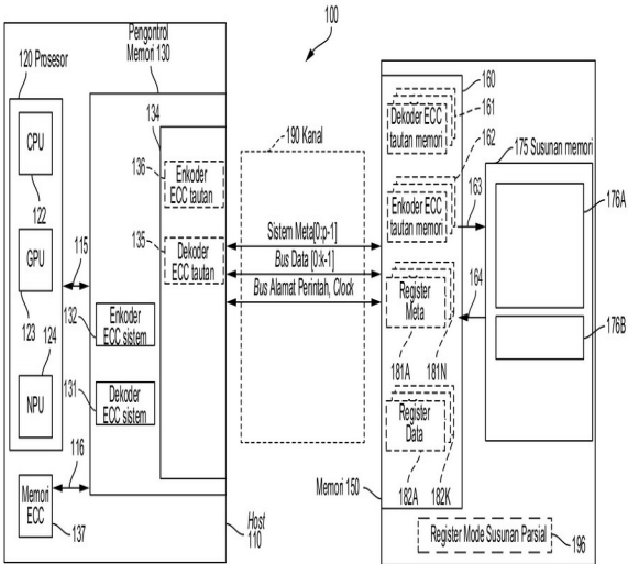
Gambar 2D
