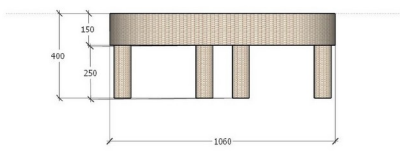
Tampak Samping
