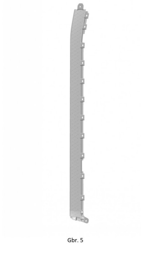
Tampak Samping
