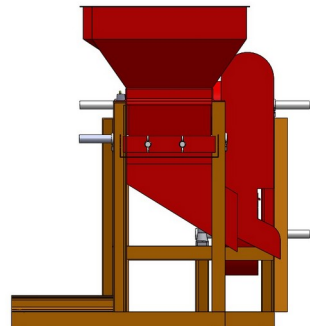
Tampak Samping
